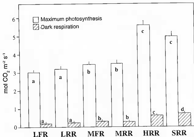
Figure 3. Maximum photosynthesis ( A_{max} ) and dark respiration ( R_{dark} ) in leaves from seedlings of the different shade treatments. Treatment symbols are described in the methods section and Table 1. Vertical bars indicate standard errors, and identical letters between treatments indicate that they are not significantly different from each other.
